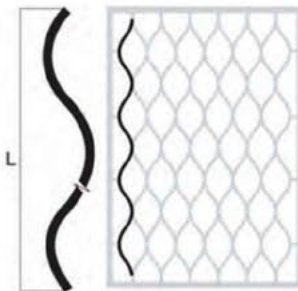
P/070-12x6 12x6, L2650, 1m 2 =5,5pcs P/070-12x12 12x12, L2600, 1m 2 =5,5pcs
