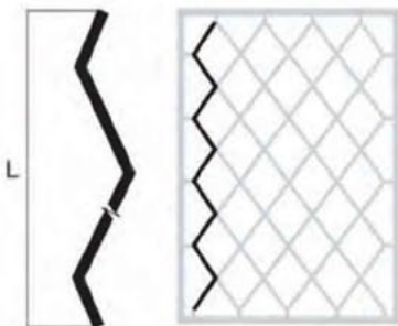
P/060-12x6 12x6, L2350, 1m 2 =5,5pcs
